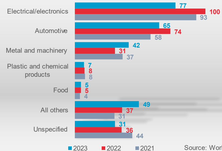
Annual installations of industrial robots by customer industry - China 1,000 units
