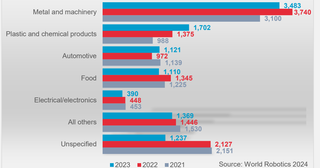
Annual installations of industrial robots by customer industry - Italy
